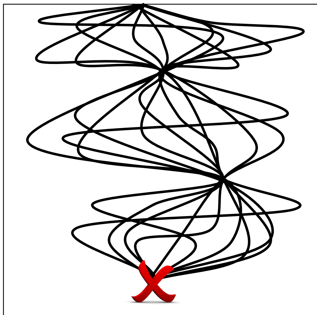
converges locally
