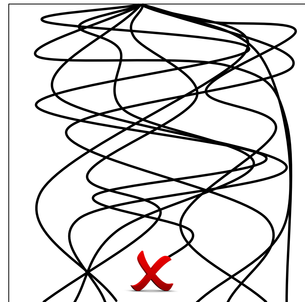
diverges globally
